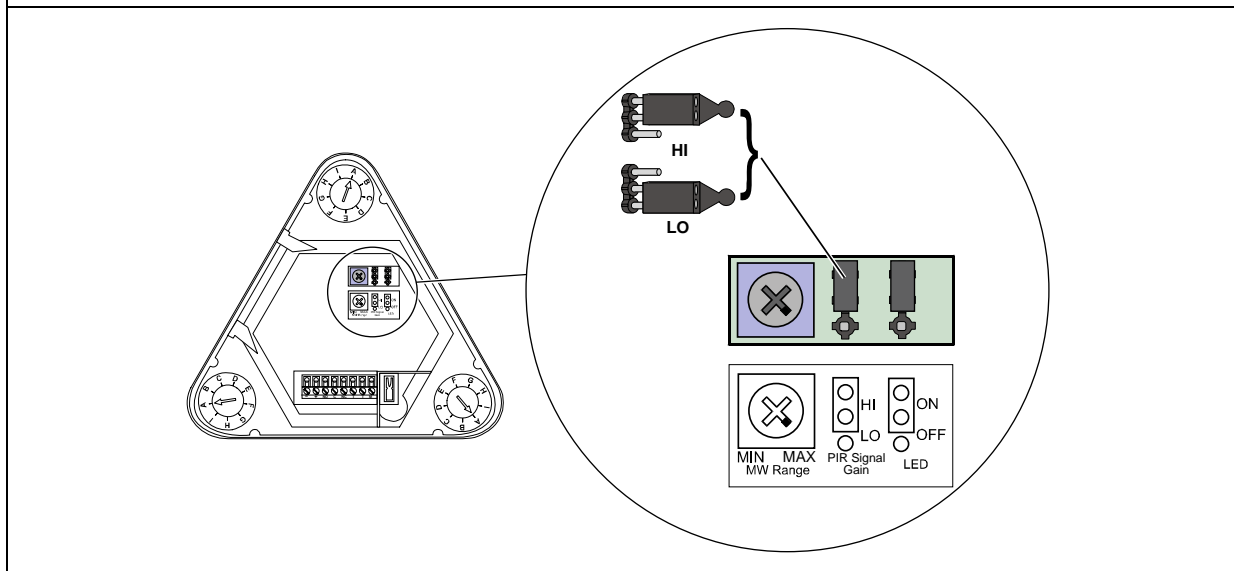
Figure 1: DS939 PIR Sensitivity Selection Pins
